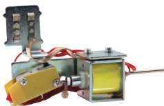
NC 1600-S
